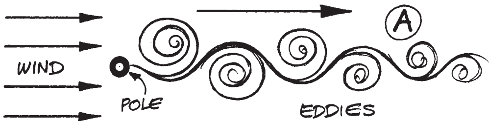
FIGURE 41 A Plan view of eddies formed as wind passes the pole. Each eddy is a cylinder roughly at right angles to the paper. B Wave shape of flag between left and right eddies.
